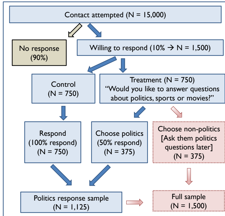
Figure 4: Selection sensitive survey design
