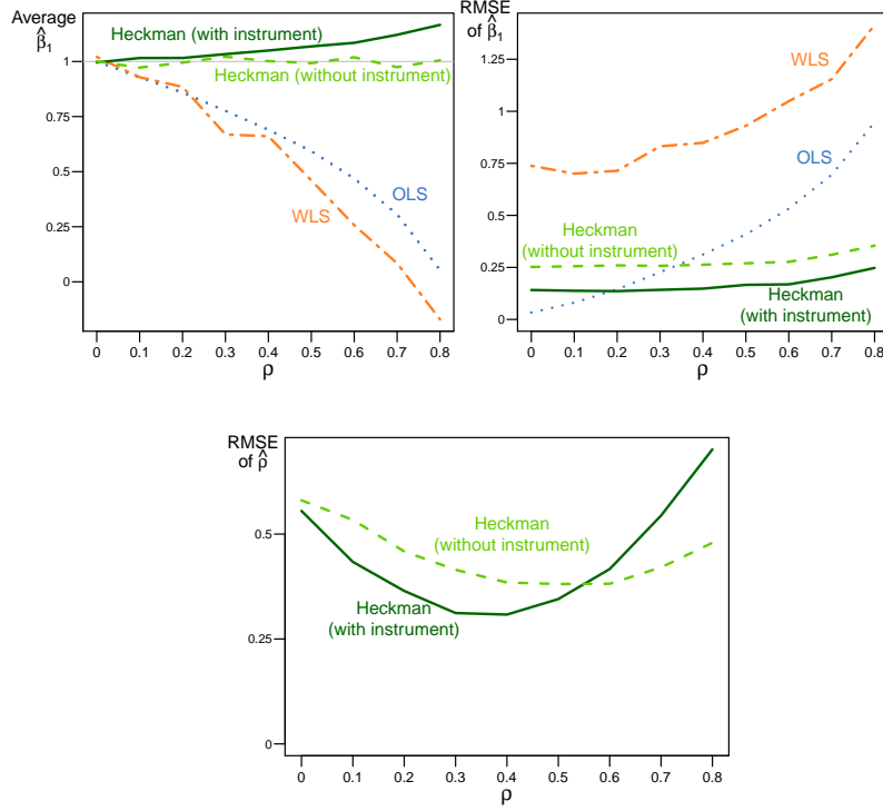
Figure 7: Simulation results for better first stage covariate ( \gamma_2 = 1.0 )
