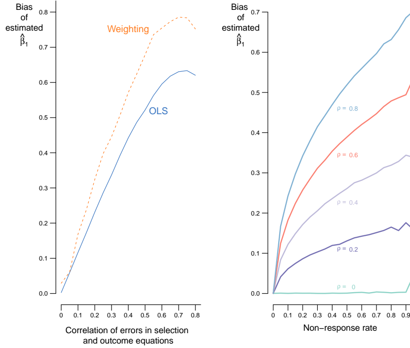
Figure 2: Bias in Weighting and OLS models
