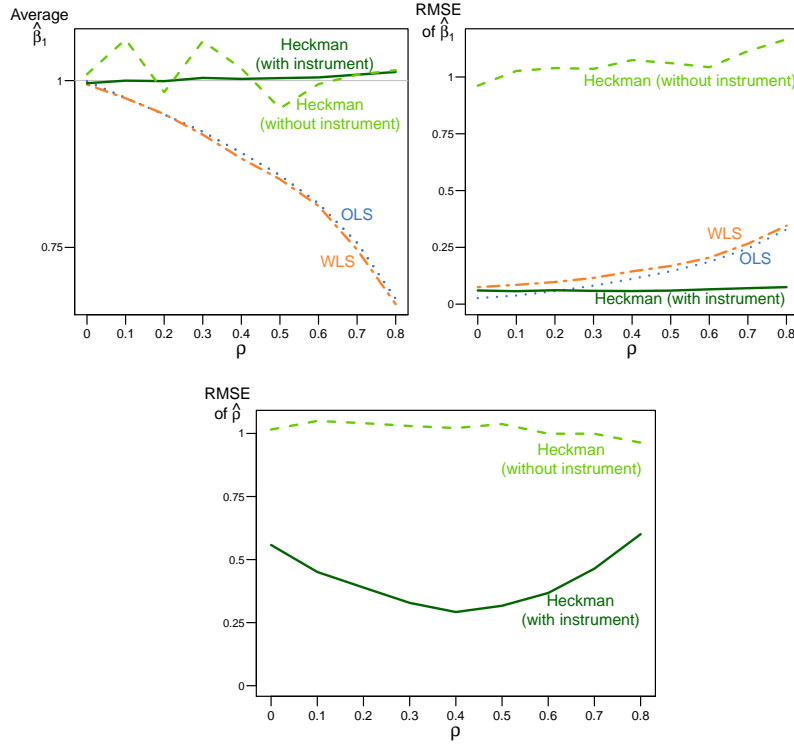
Figure 6: Simulation results for weak first stage covariate ( \gamma_2 = 0.3 )
