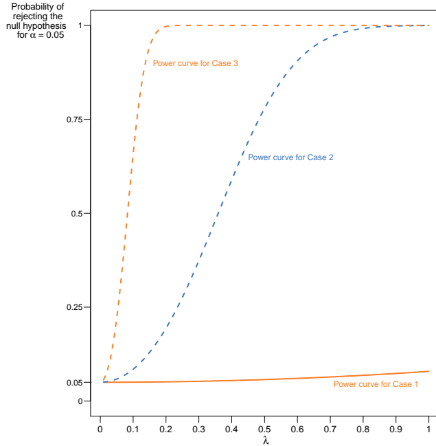
Figure B.3: Power curve for H_0: \lambda = 0 for three values of \gamma and N = 2,500
