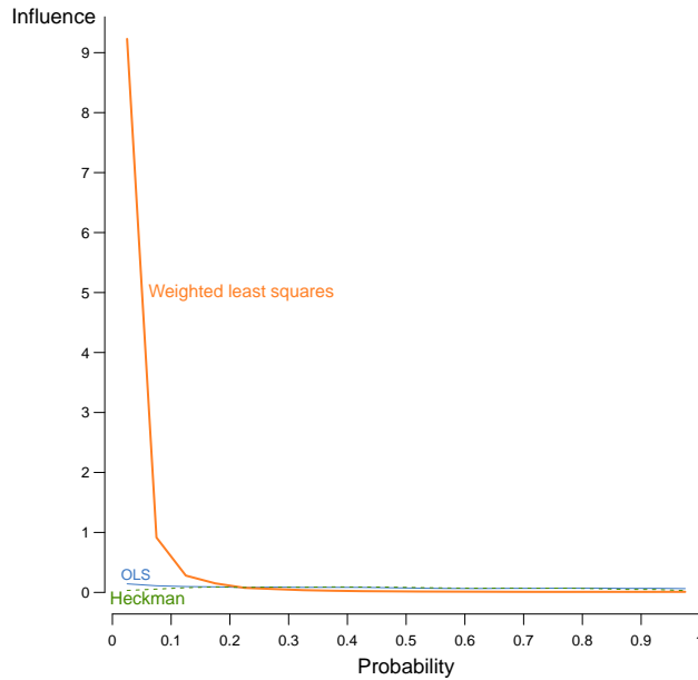
Figure A.1: Influence in OLS, weighting and Heckman models
